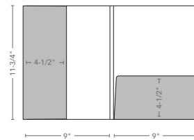
Horizontal and Vertical Pockets with 3/8" Spine Die #275 40 sheet capacity 9-1/2" x 12-1/2" envelope Optional card cuts
