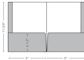
Two Standard Pockets Die #259 30 sheet capacity 9-1/2" x 12-1/2" envelope Optional card cuts Turn-ins under pockets
