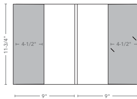
Two Vertical Pockets with 3/8" Spine Die #280 40 sheet capacity 9-1/2" x 12-1/2" envelope Business card cuts built into right pocket
