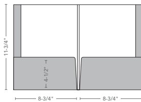
Two Standard Pockets Die #204 30 sheet capacity 9" x 12" envelope Optional card cuts Turn-ins under pockets
