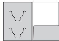
Die #246 12 pt CD slits left 8-3/4" (w) x 11-3/4" (h) x 1/4" (s) Holds 8-1/2" x 11" materials
