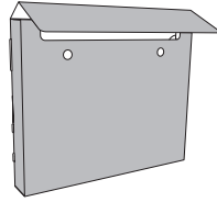
Die #317: 1" deep, 18 pt Die #318: 1-1/2" deep, 24 pt Die #319: 2" deep, 24 pt 11-1/4" (w) x 9-1/8" (h) 2 Velcro® closures
