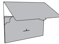
Die #332 1/4" deep, 12 pt 11-1/4" (w) x 9-3/16" (h) Tuck closure
