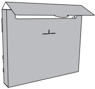
Die #314: 1" deep, 18 pt Die #315: 1-1/2" deep, 24 pt Die #316: 2" deep, 24 pt 11-1/4" (w) x 9-1/8" (h) Tuck closure
