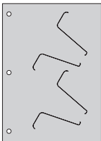
Die #408 12 pt CD slits 7-1/8" (w) x 10" (h)
