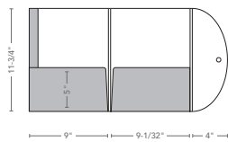
Rounded Portfolio with 1/4" Spine Die #266 40 sheet capacity 9-1/2" x 12-1/2" envelope Optional card cuts 1 Velcro® closure
