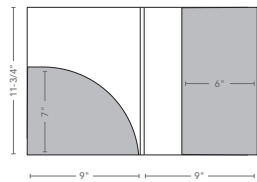
Round and Vertical Pockets with 5/16" Spine Die #274 40 sheet capacity 9-1/2" x 12-1/2" envelope Optional card cuts
