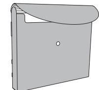
Die #329: 1" deep, 18 pt Die #330: 1-1/2" deep, 24 pt Die #331: 2" deep, 24 pt 11-1/4" (w) x 9-1/8" (h) 1 Velcro® closure
