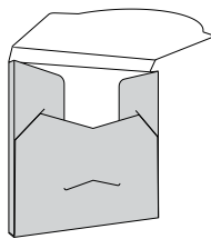
Die #10901 Four Flap Enclosure 12 pt 4-7/8" x 4-7/8" x 1/2" Tuck Closure
