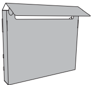
Die #326: 1" deep, 18 pt Die #327: 1-1/2" deep, 24 pt Die #328: 2" deep, 24 pt 11-1/4" (w) x 9-1/8" (h) Tuck closure
